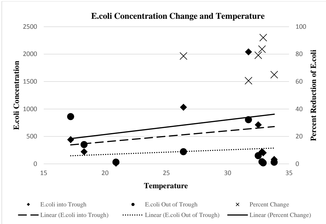
Figure 5.28 Relation between Water Temperature and E. coli Concentration Change in Trough 2
